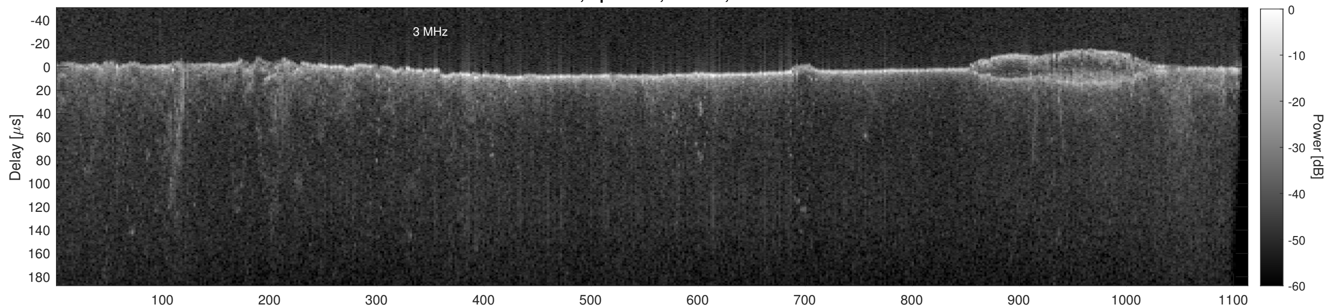
Orbit 16282, Cluttergram
