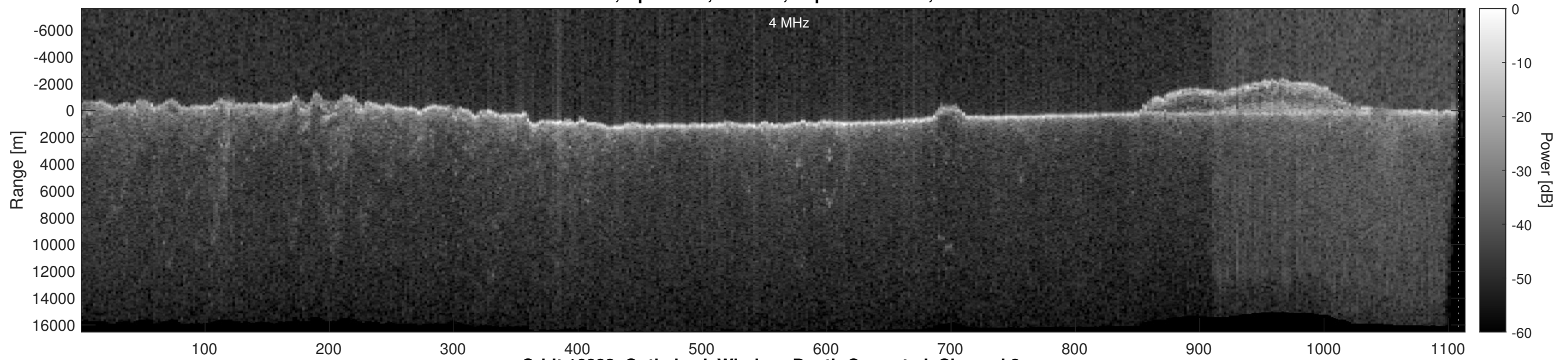
Orbit 16282, Optimized, Window, Depth-Corrected, Channel 2
