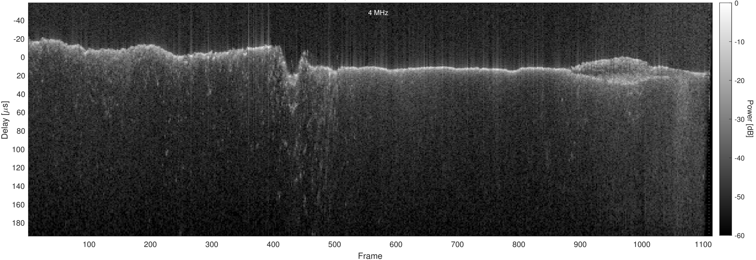
Orbit 16285, Chapman, No Window, Channel 2
