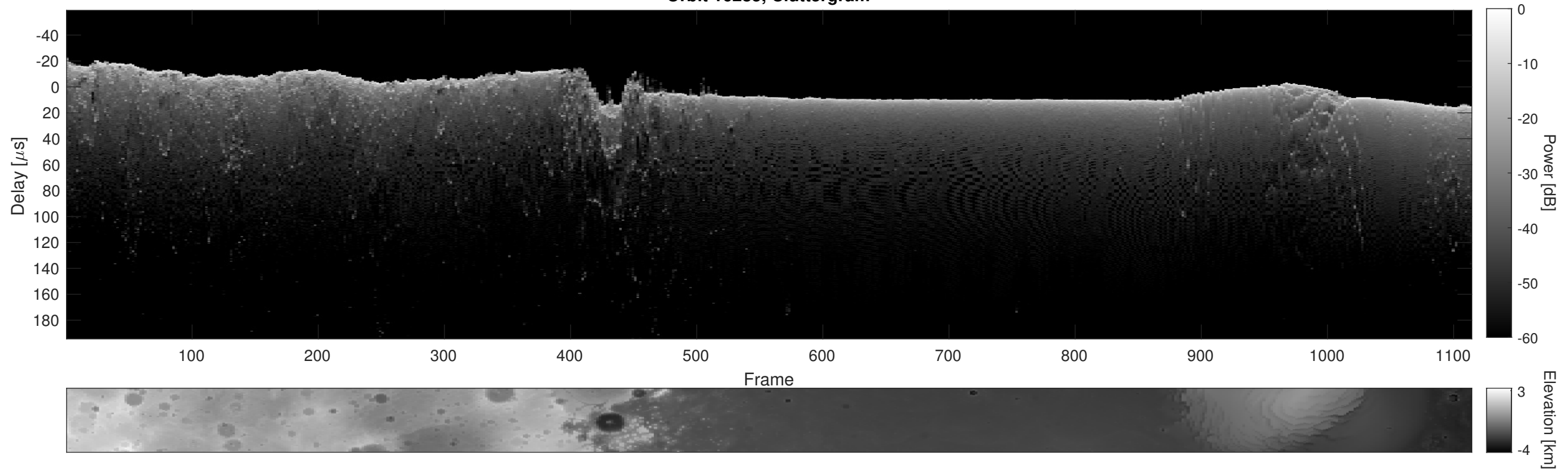
Orbit 16285, Cluttergram
