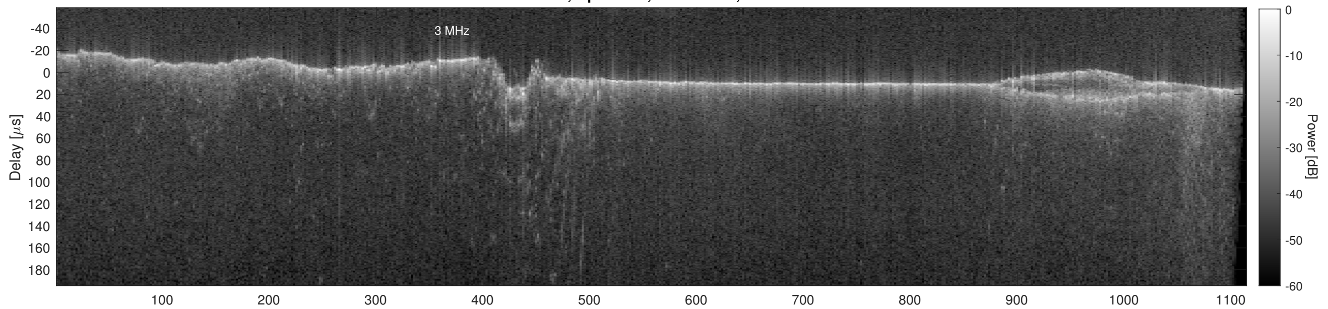
Orbit 16285, Cluttergram
