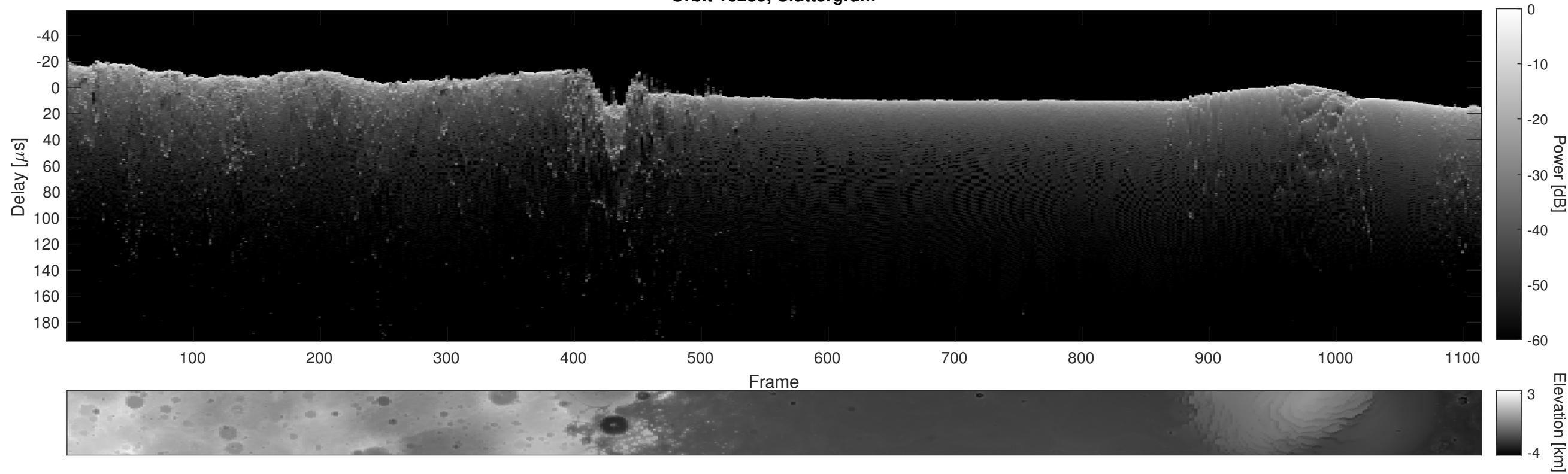
Orbit 16285, Cluttergram
