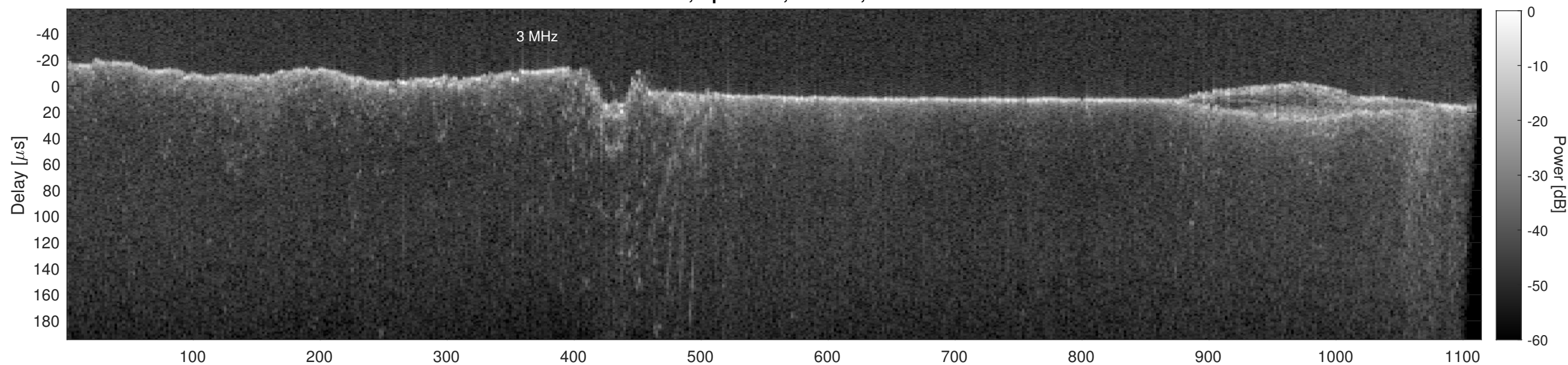
Orbit 16285, Cluttergram
