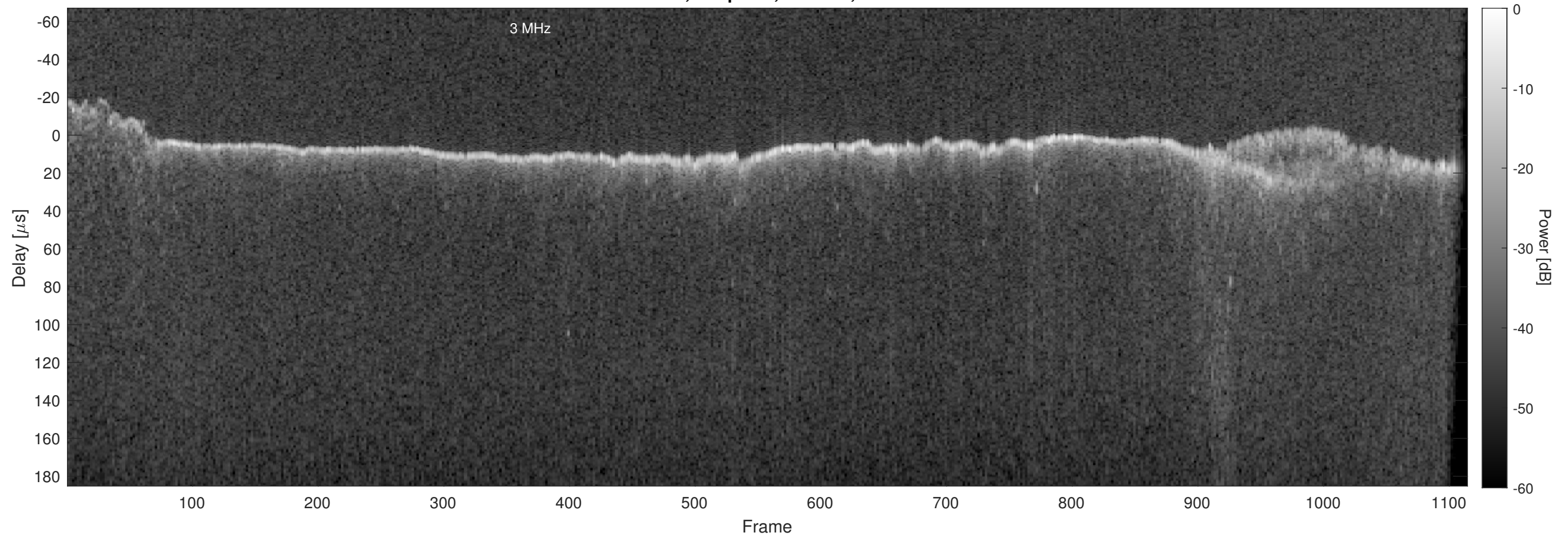
Orbit 16288, Chapman, Window, Channel 2
