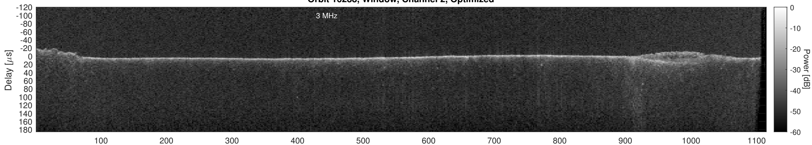
Orbit 16288, Cluttergram
