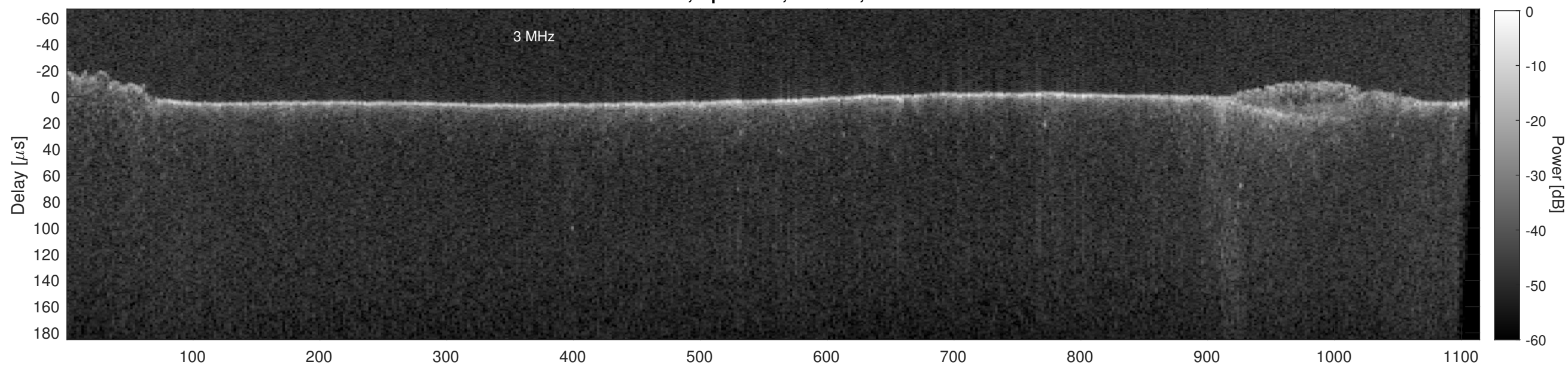
Orbit 16288, Cluttergram
