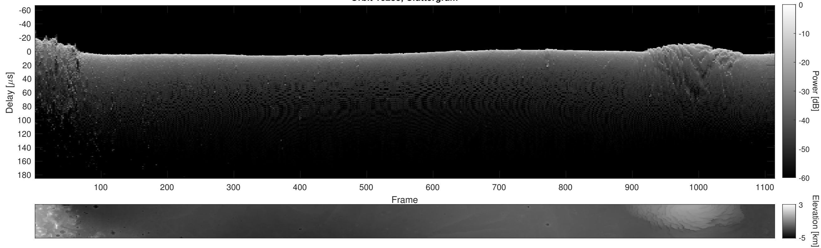
Orbit 16288, Cluttergram
