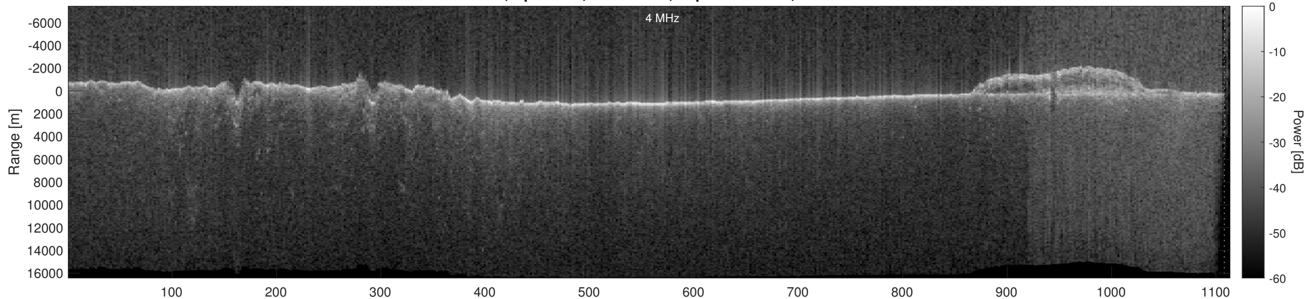
Orbit 16289, Optimized, No Window, Depth-Corrected, Channel 2
