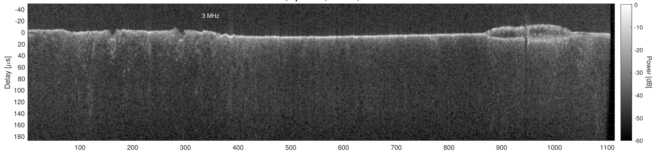
Orbit 16289, Cluttergram
