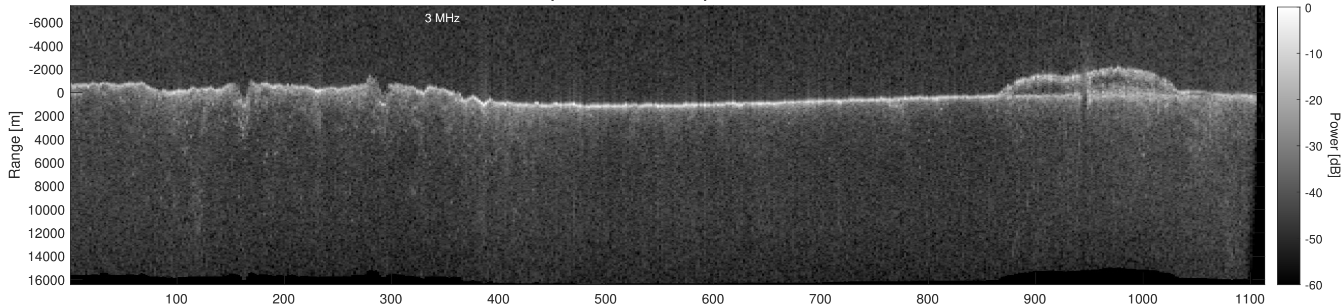
Orbit 16289, Depth-Corrected Cluttergram
