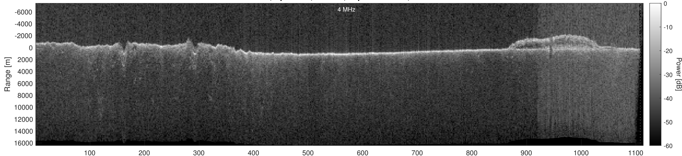
Orbit 16289, Optimized, Window, Depth-Corrected, Channel 2
