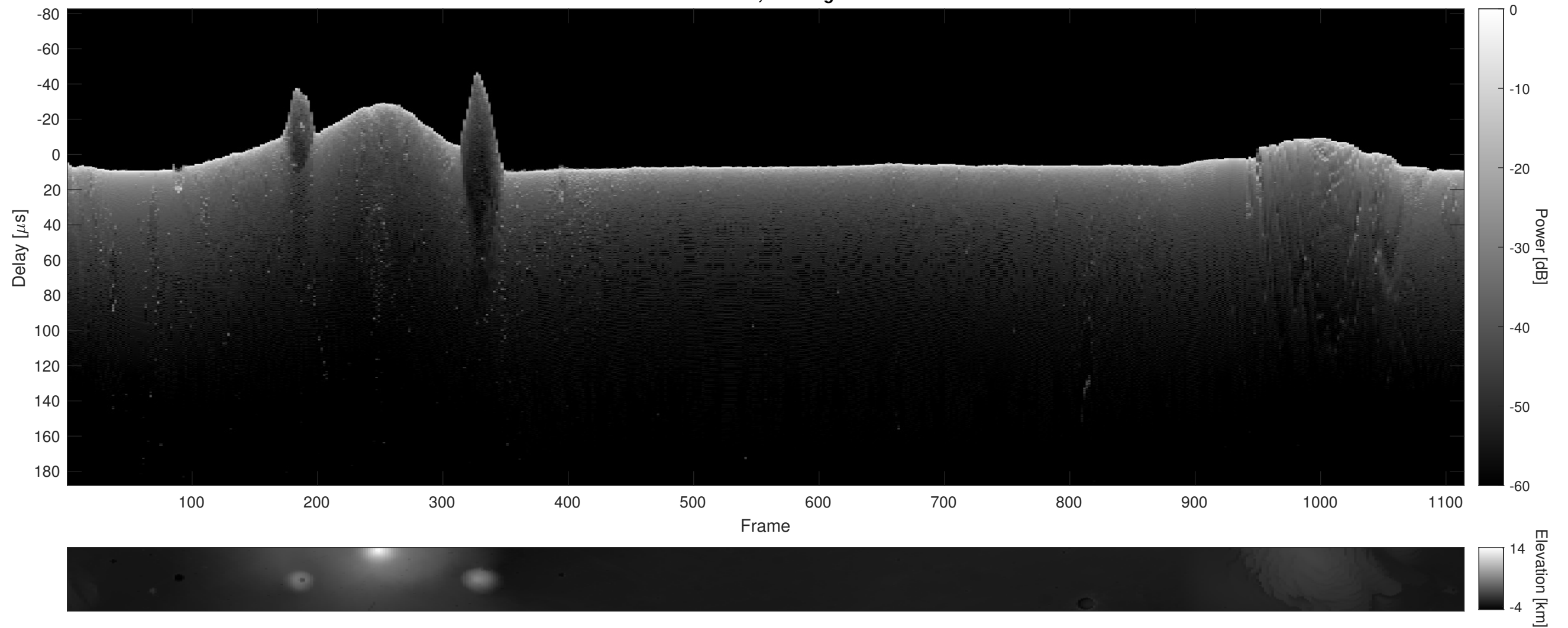
Orbit 16291, Cluttergram
