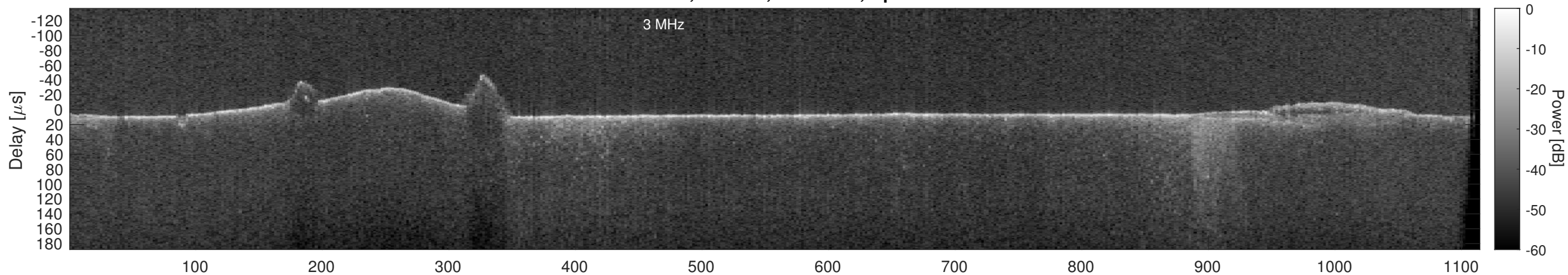
Orbit 16291, Cluttergram
