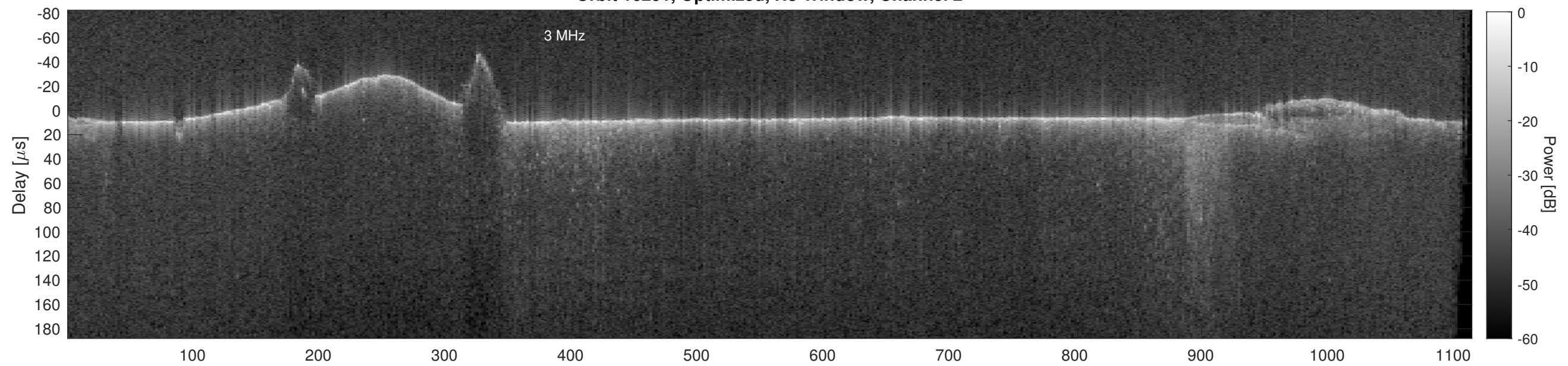
Orbit 16291, Cluttergram
