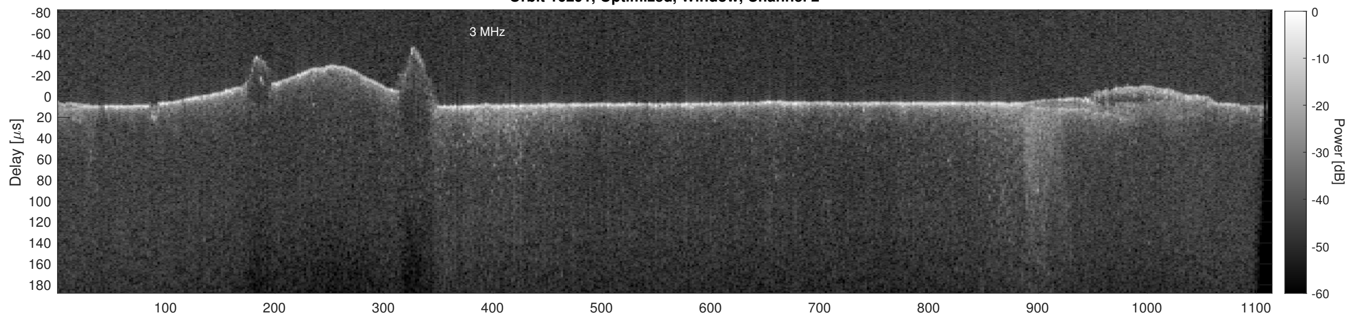
Orbit 16291, Cluttergram
