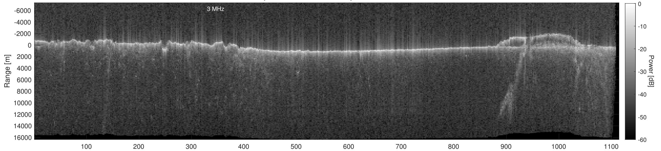
Orbit 16296, Depth-Corrected Cluttergram
