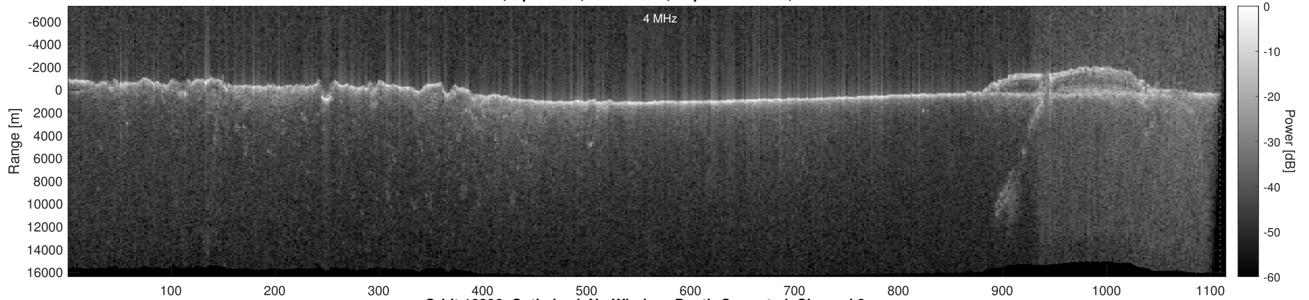
Orbit 16296, Optimized, No Window, Depth-Corrected, Channel 2
