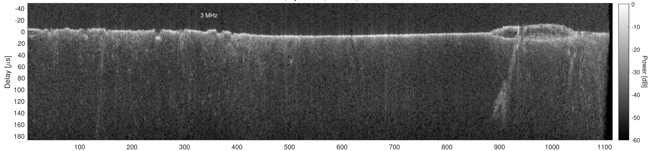
Orbit 16296, Cluttergram
