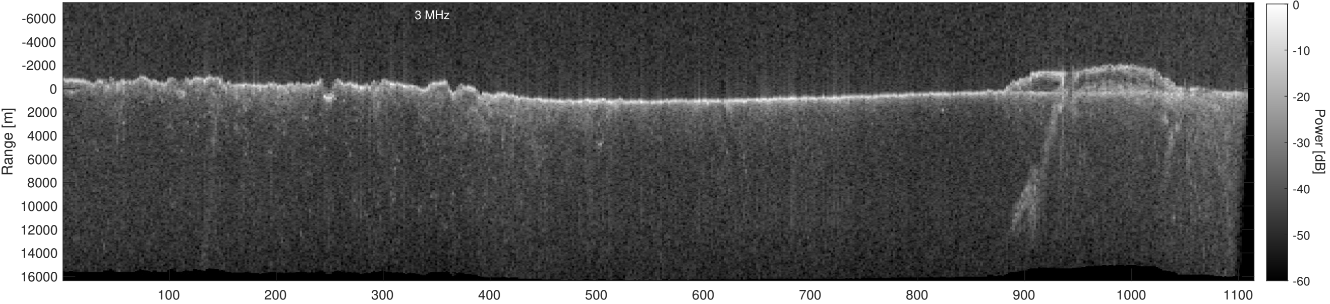
Orbit 16296, Depth-Corrected Cluttergram
