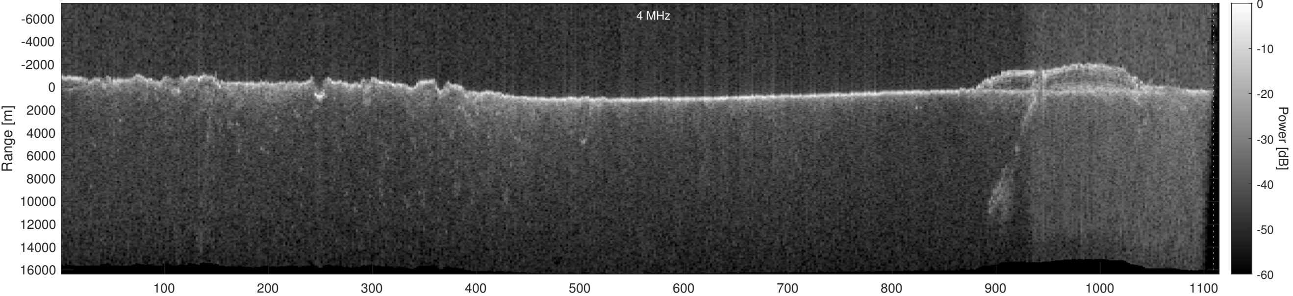
Orbit 16296, Optimized, Window, Depth-Corrected, Channel 2
