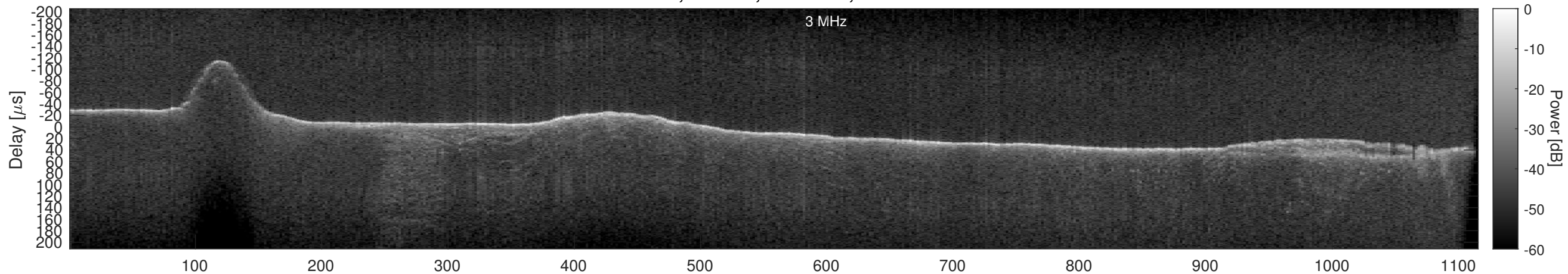
Orbit 16297, Window, Channel 2, Chapman
