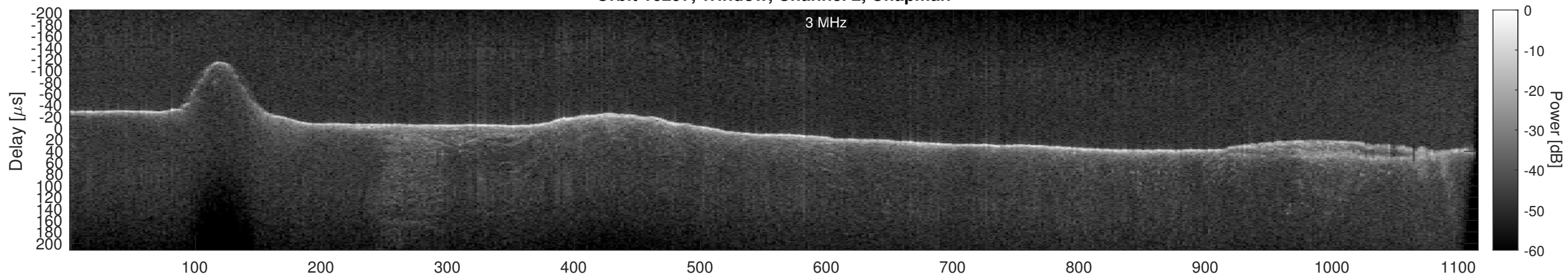
Orbit 16297, Window, Channel 2, Optimized
