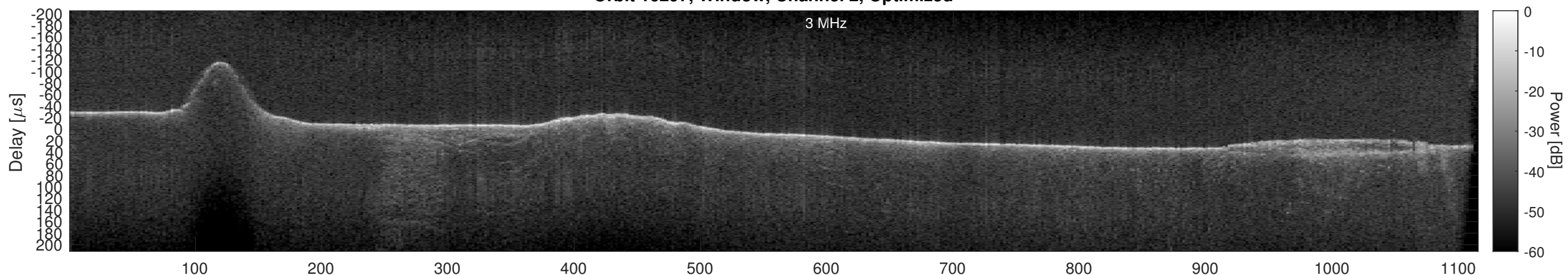
Orbit 16297, Cluttergram
