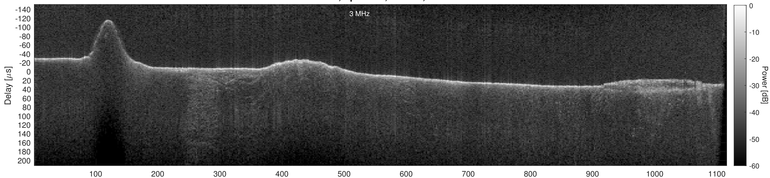
Orbit 16297, Cluttergram
