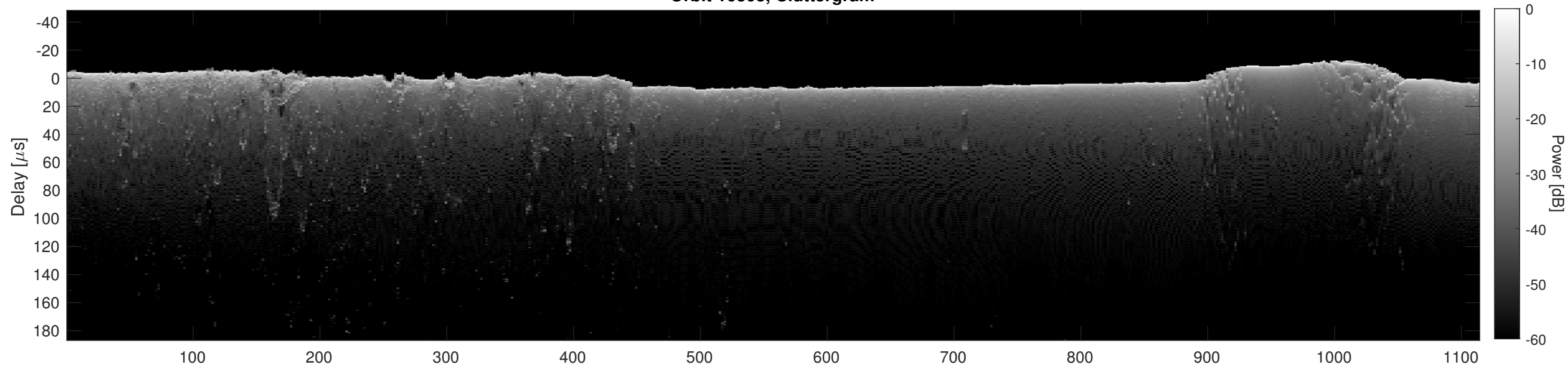
Orbit 16303, Cluttergram
