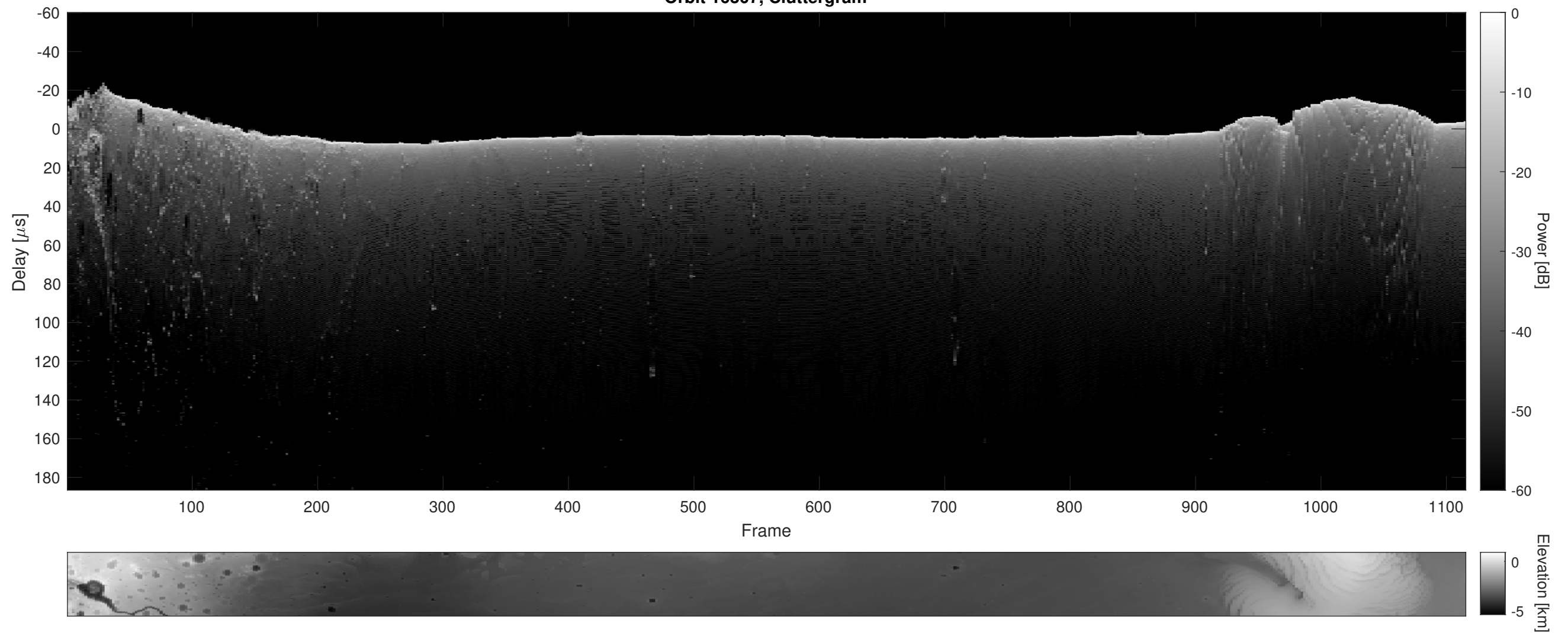
Orbit 16307, Cluttergram
