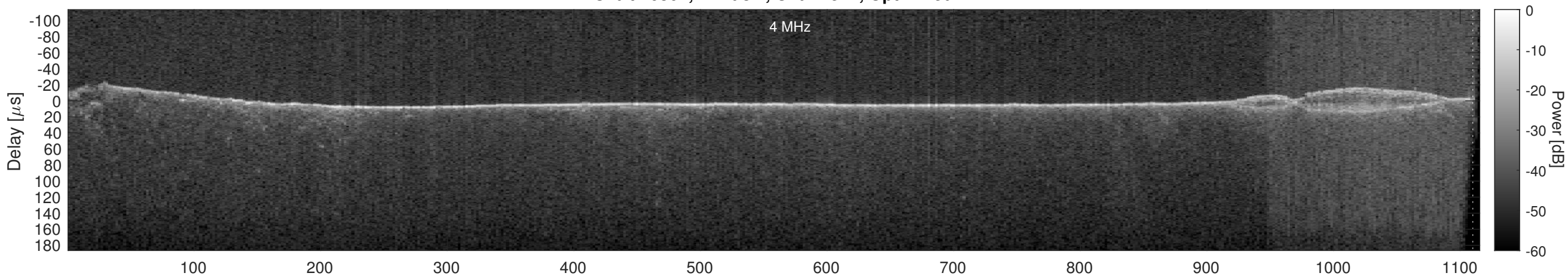
Orbit 16307, Cluttergram
