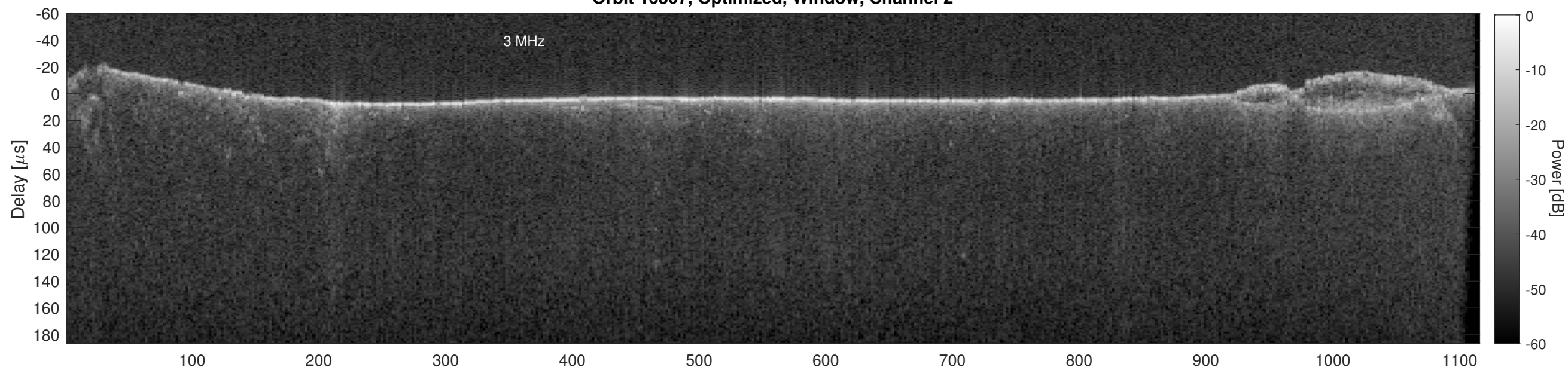
Orbit 16307, Cluttergram
