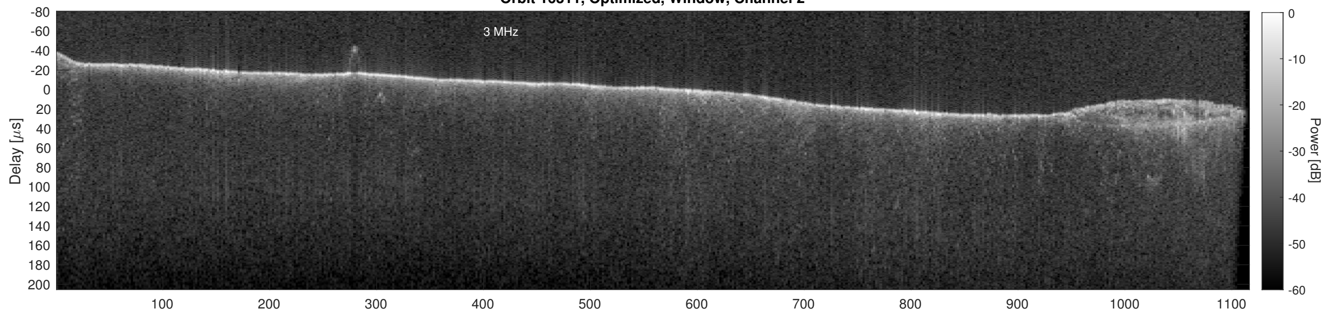
Orbit 16311, Cluttergram
