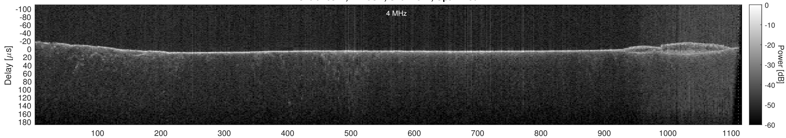
Orbit 16314, Cluttergram
