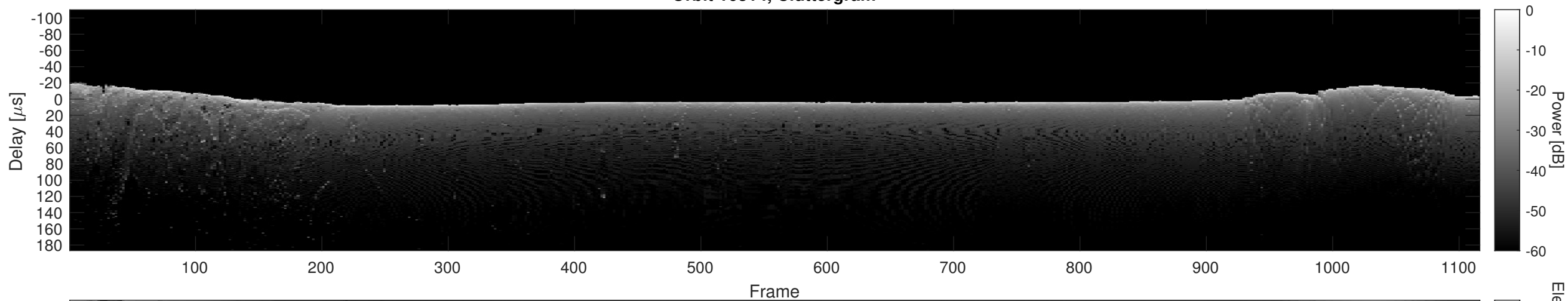
Orbit 16314, Cluttergram
