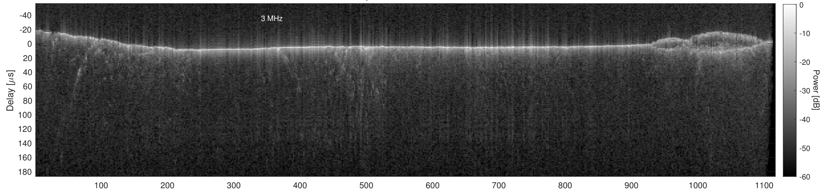
Orbit 16314, Cluttergram
