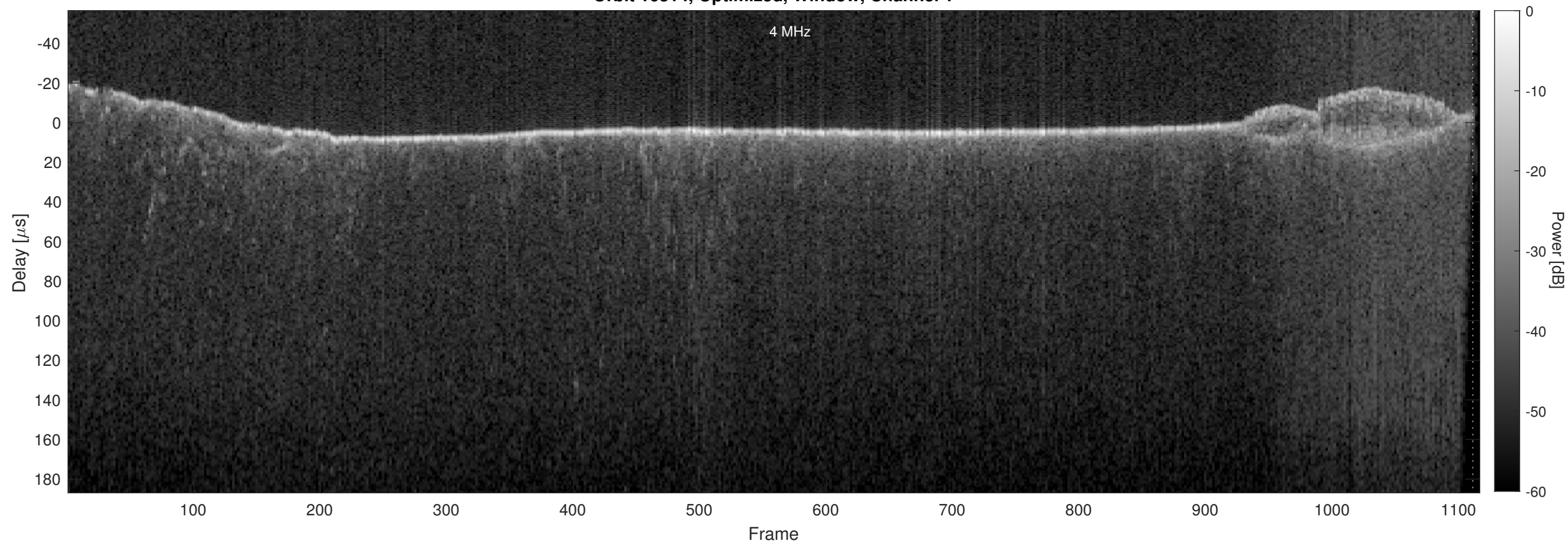
Orbit 16314, Optimized, Window, Channel 2
