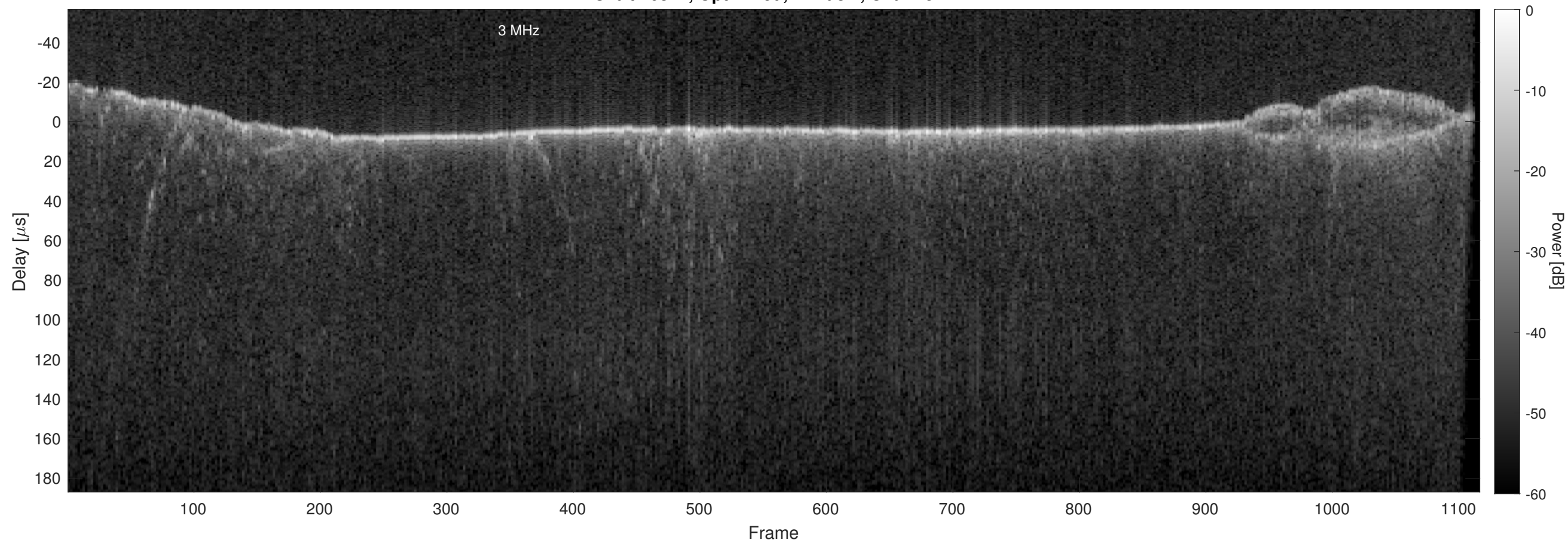
Orbit 16314, Optimized, Window, Channel 2
