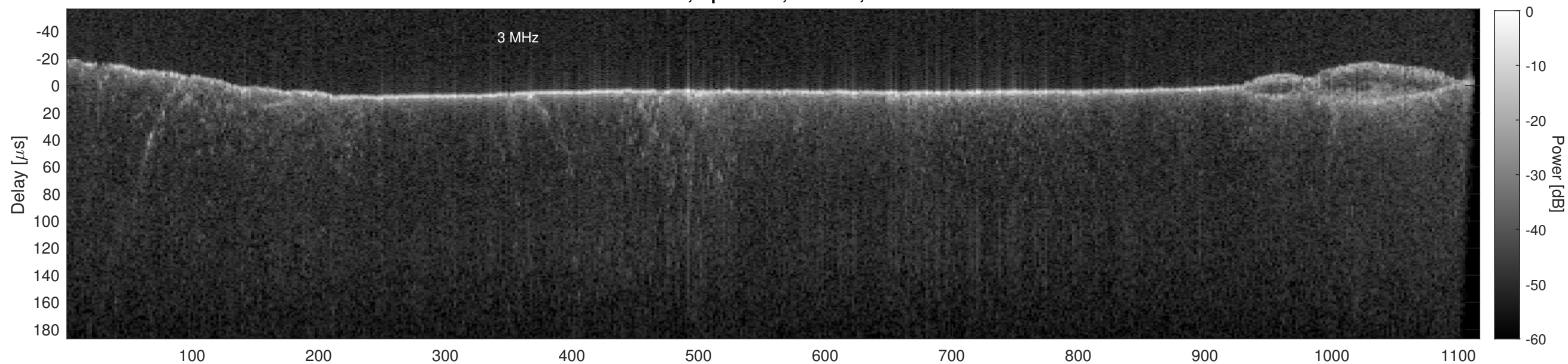
Orbit 16314, Cluttergram
