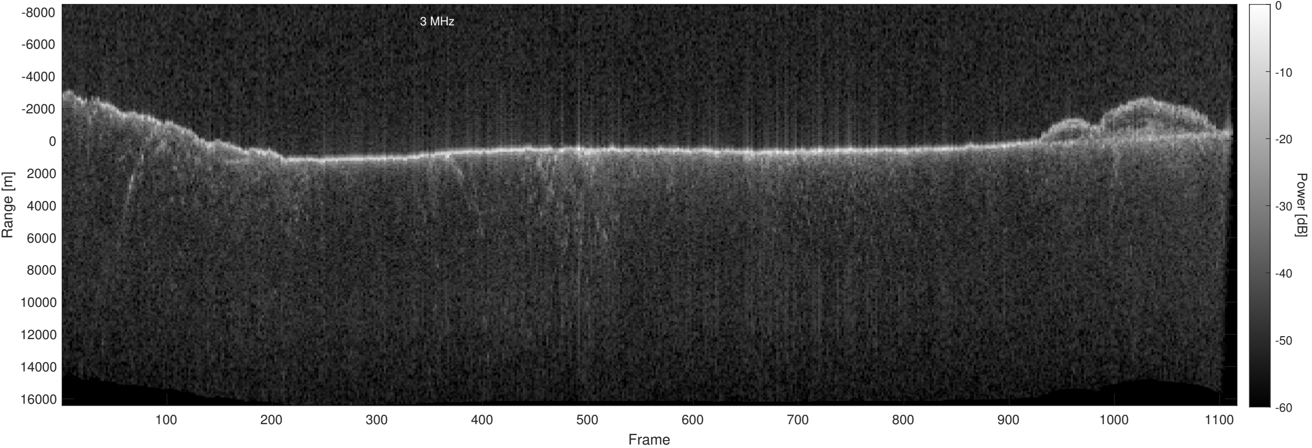
Orbit 16314, Optimized, Window, Depth-Corrected, Channel 2
