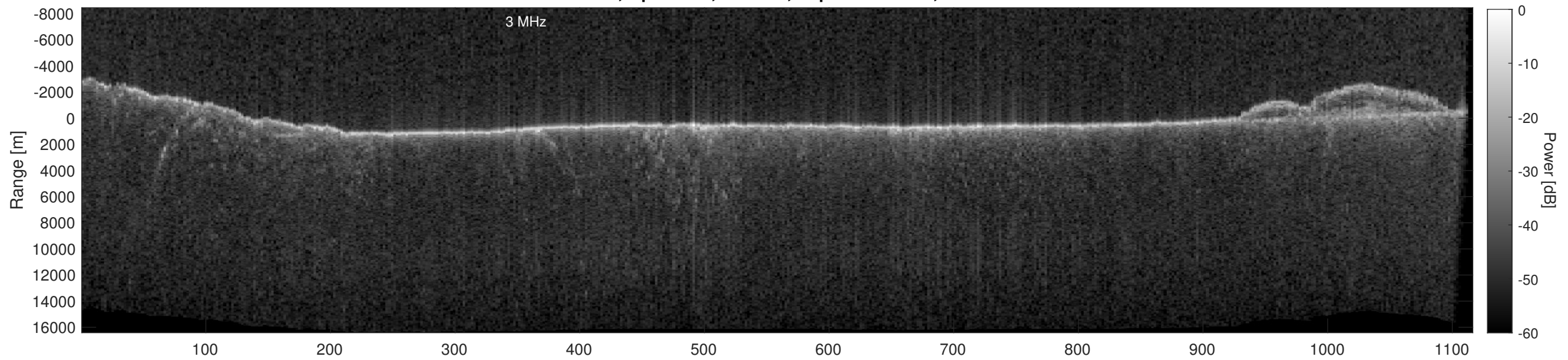
Orbit 16314, Depth-Corrected Cluttergram
