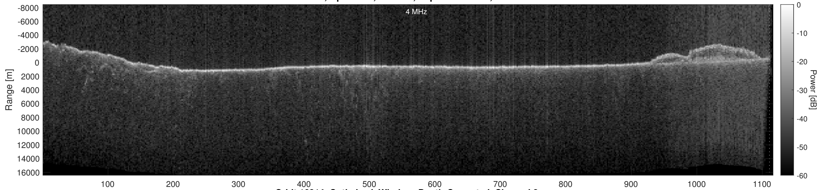
Orbit 16314, Optimized, Window, Depth-Corrected, Channel 2
