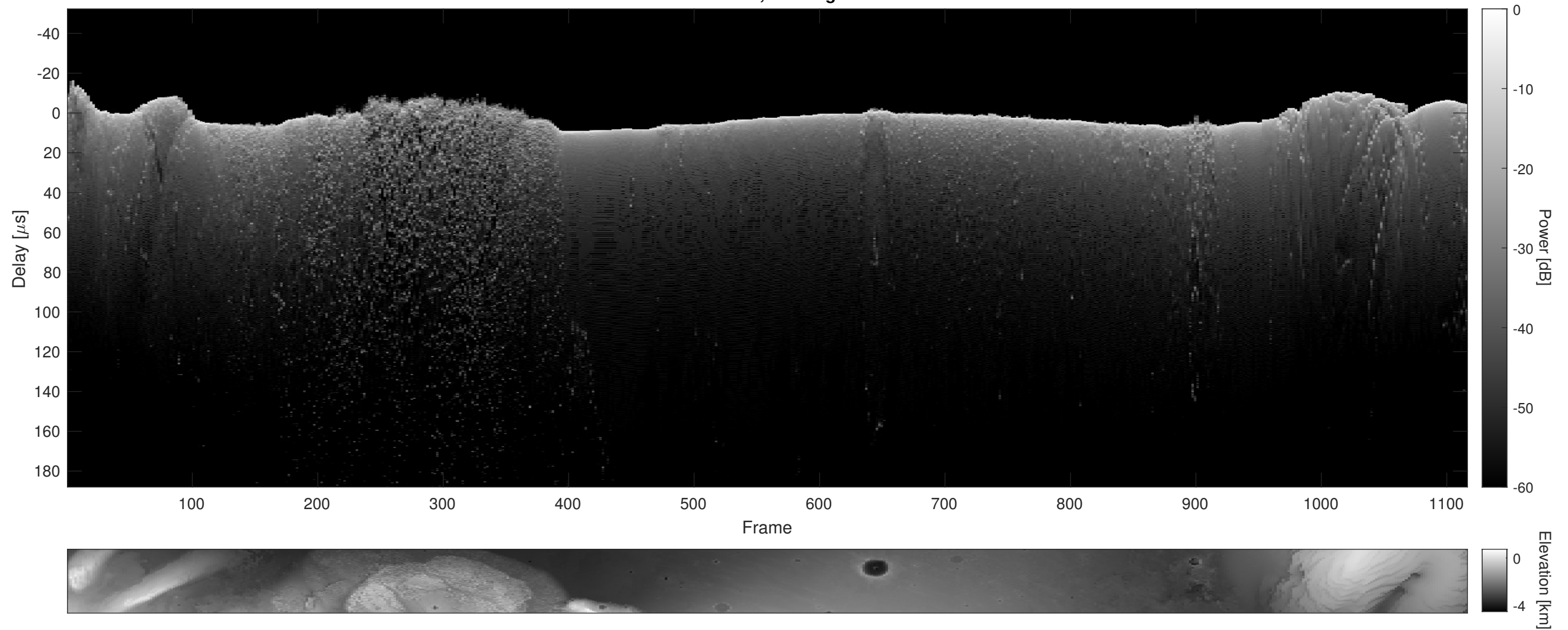
Orbit 16315, Cluttergram
