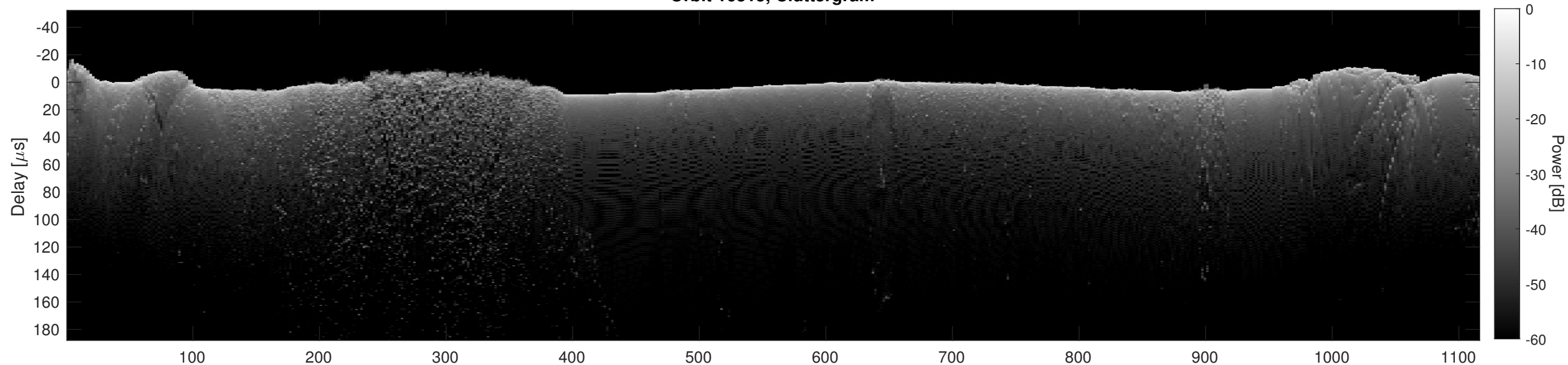
Orbit 16315, Cluttergram
