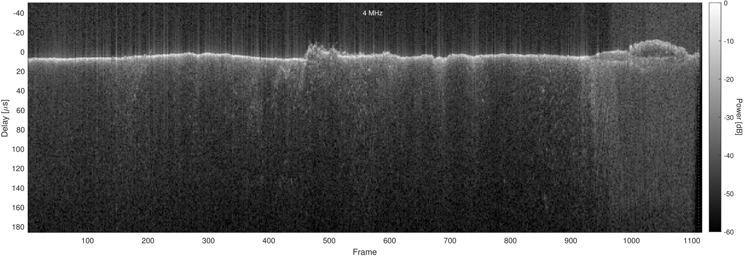
Orbit 16319, Chapman, No Window, Channel 2
