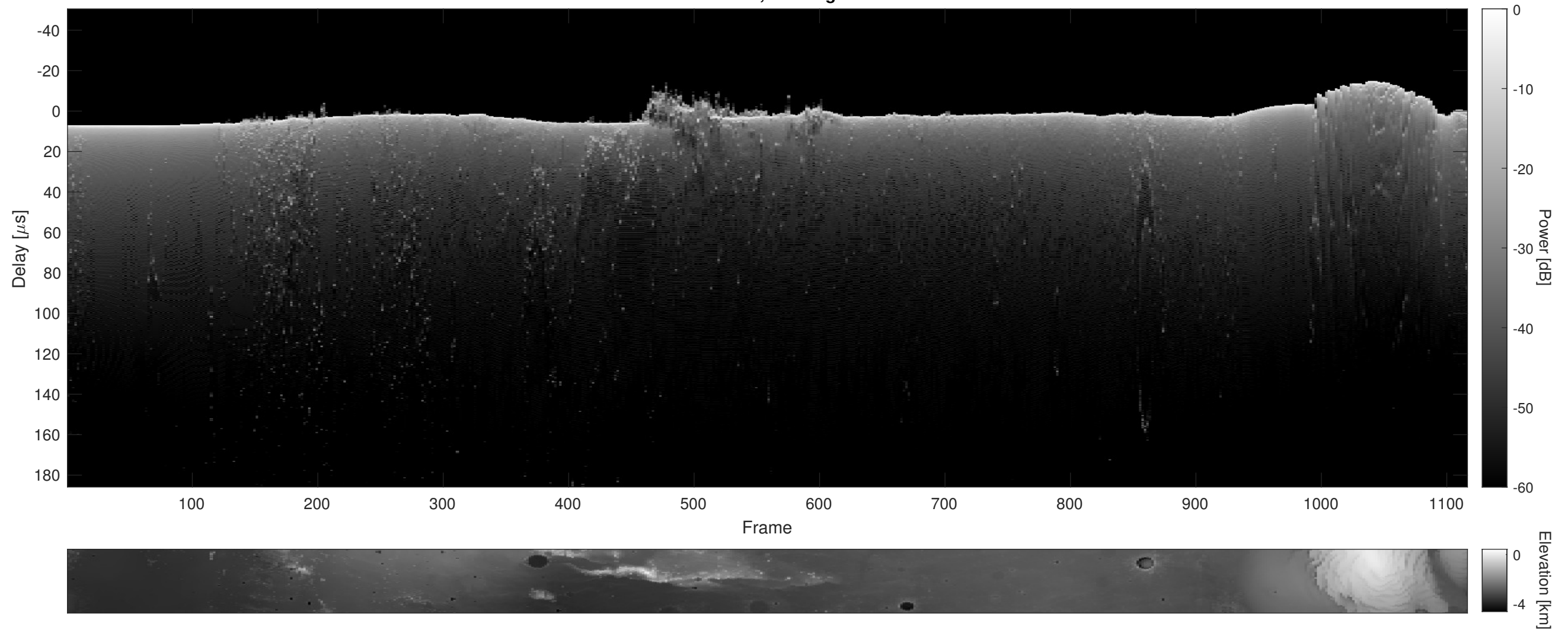
Orbit 16319, Cluttergram
