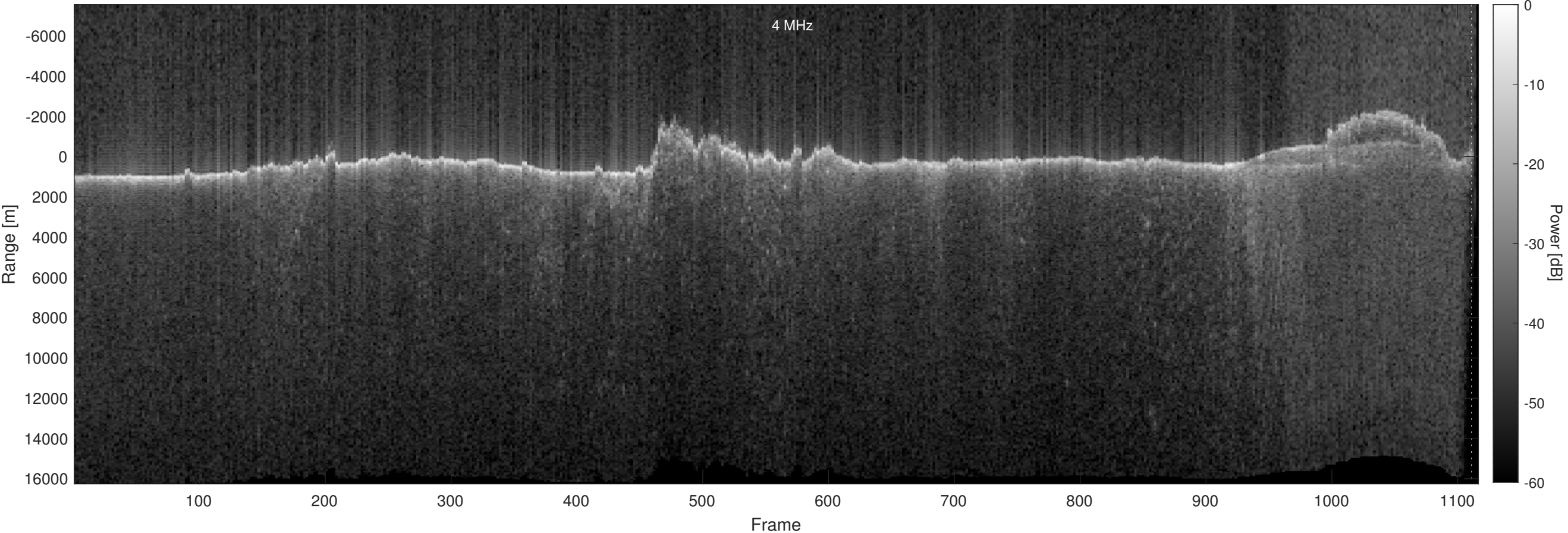
Orbit 16319, Optimized, No Window, Depth-Corrected, Channel 2
