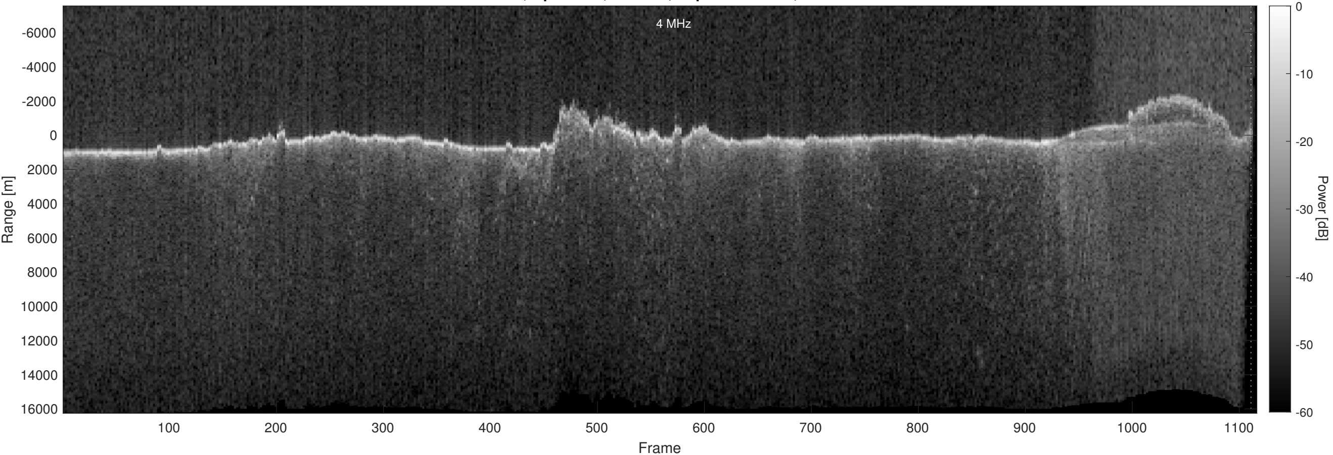
Orbit 16319, Optimized, Window, Depth-Corrected, Channel 2
