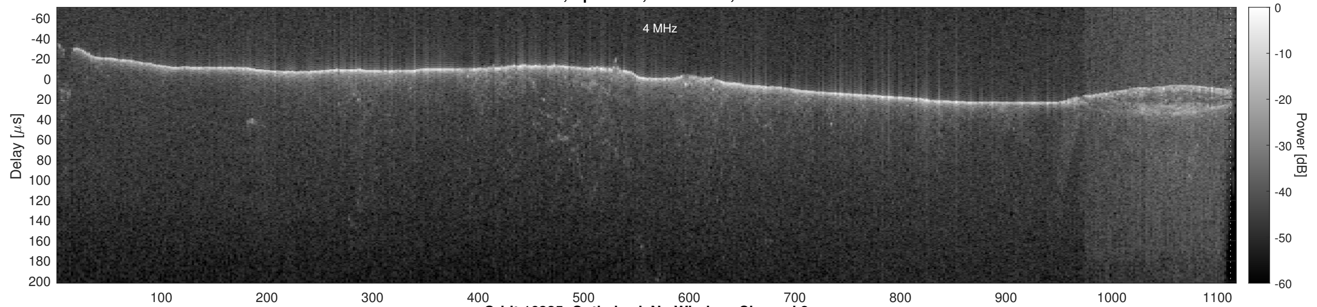
Orbit 16325, Optimized, No Window, Channel 2
