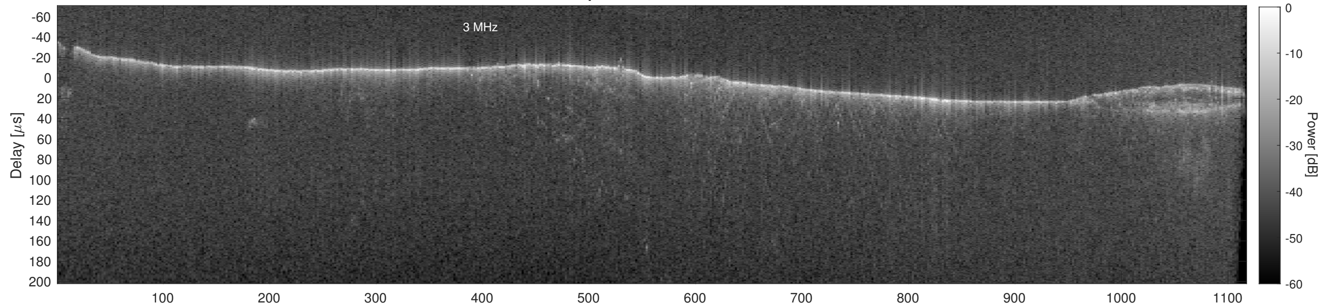
Orbit 16325, Cluttergram
