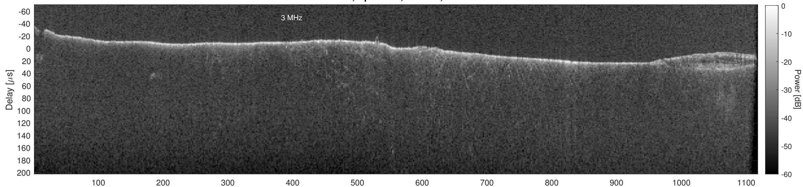
Orbit 16325, Cluttergram
