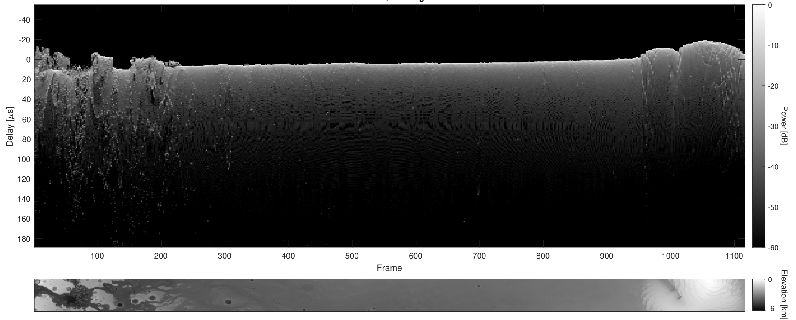
Orbit 16328, Cluttergram
