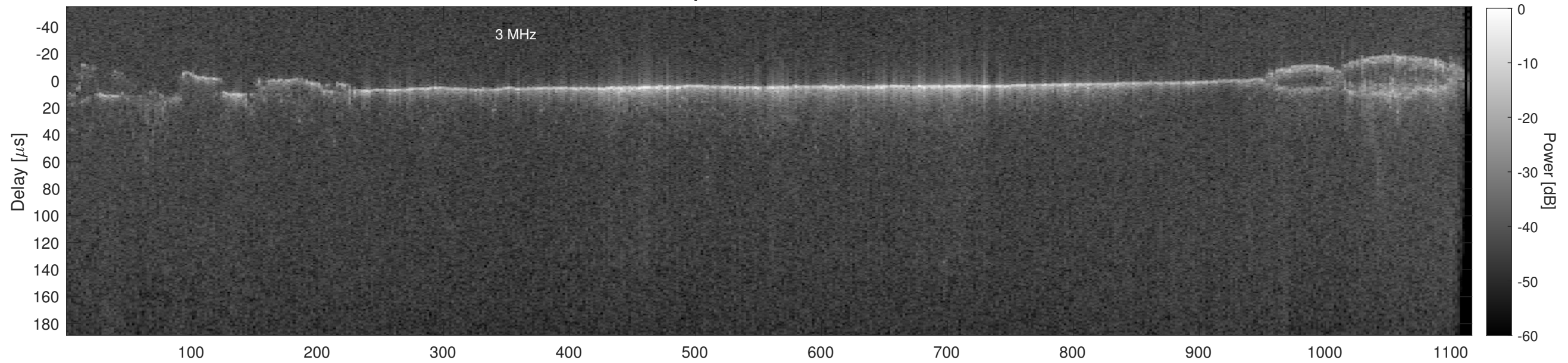
Orbit 16328, Cluttergram
