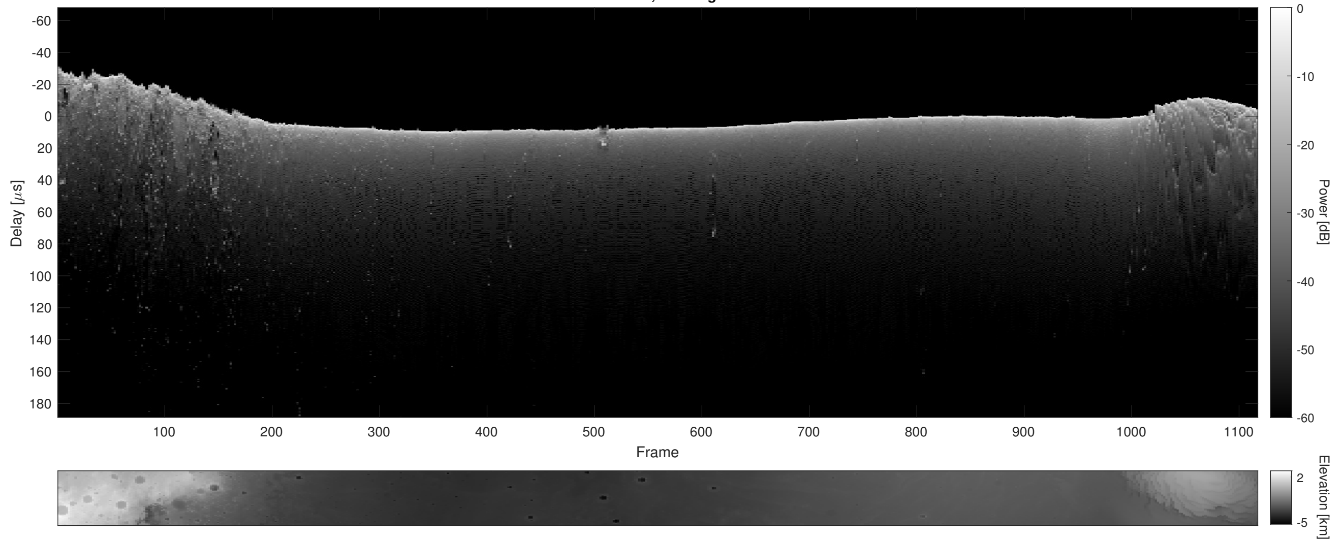
Orbit 16330, Cluttergram
