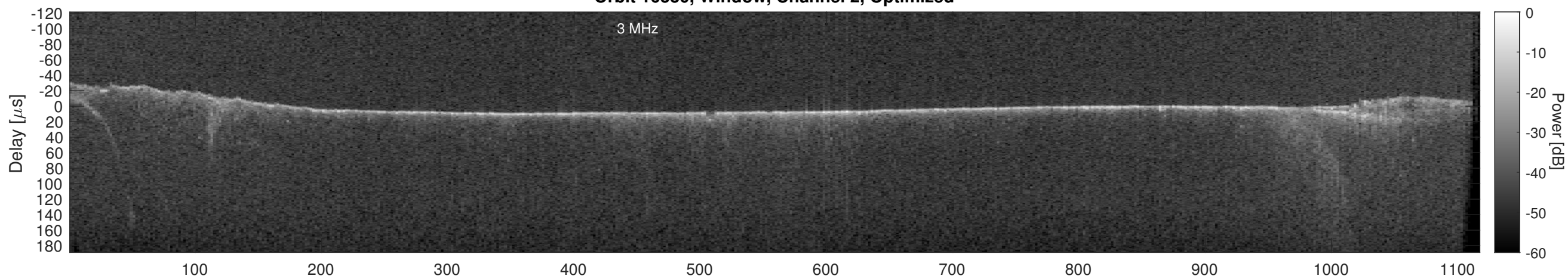
Orbit 16330, Cluttergram
