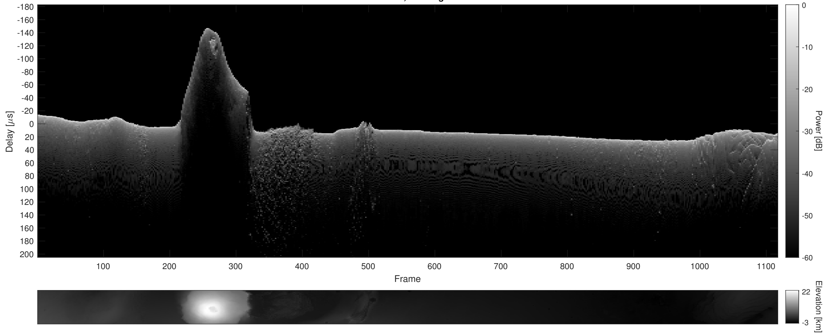
Orbit 16336, Cluttergram
