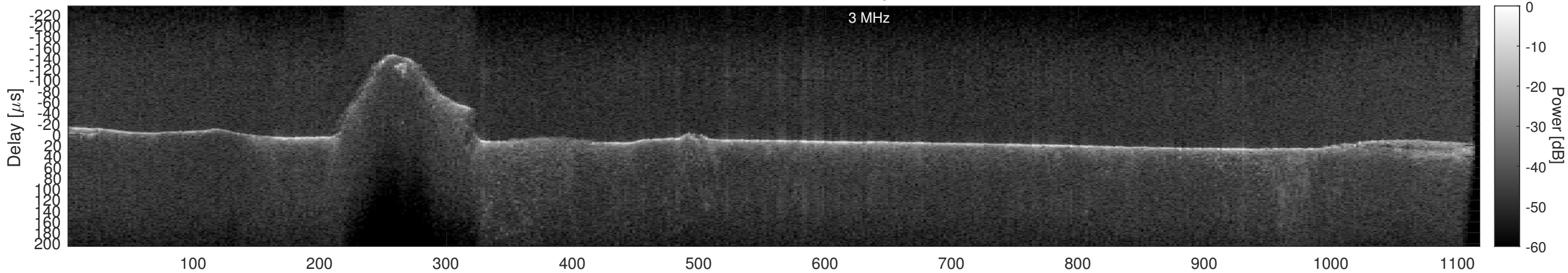
Orbit 16336, Cluttergram
