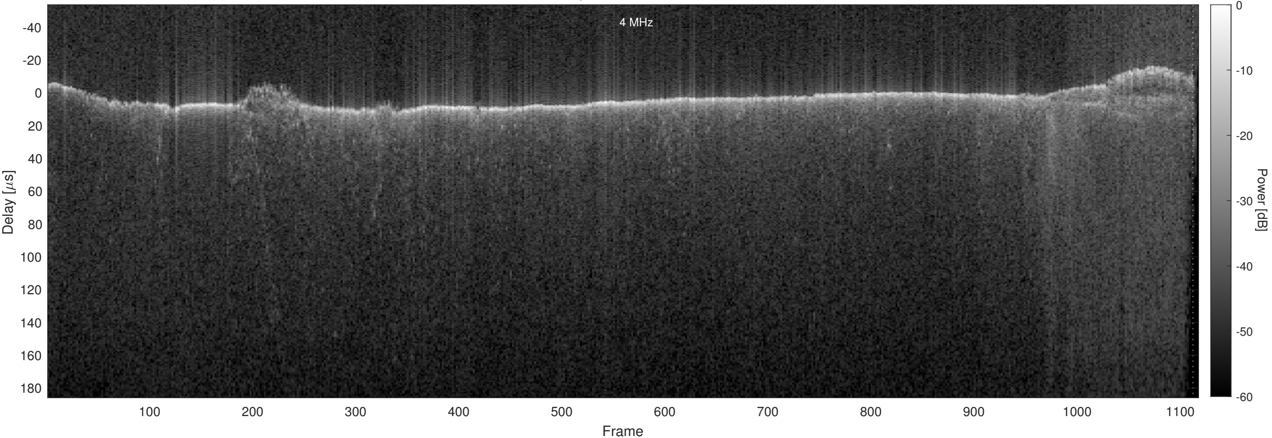
Orbit 16340, Chapman, No Window, Channel 2
