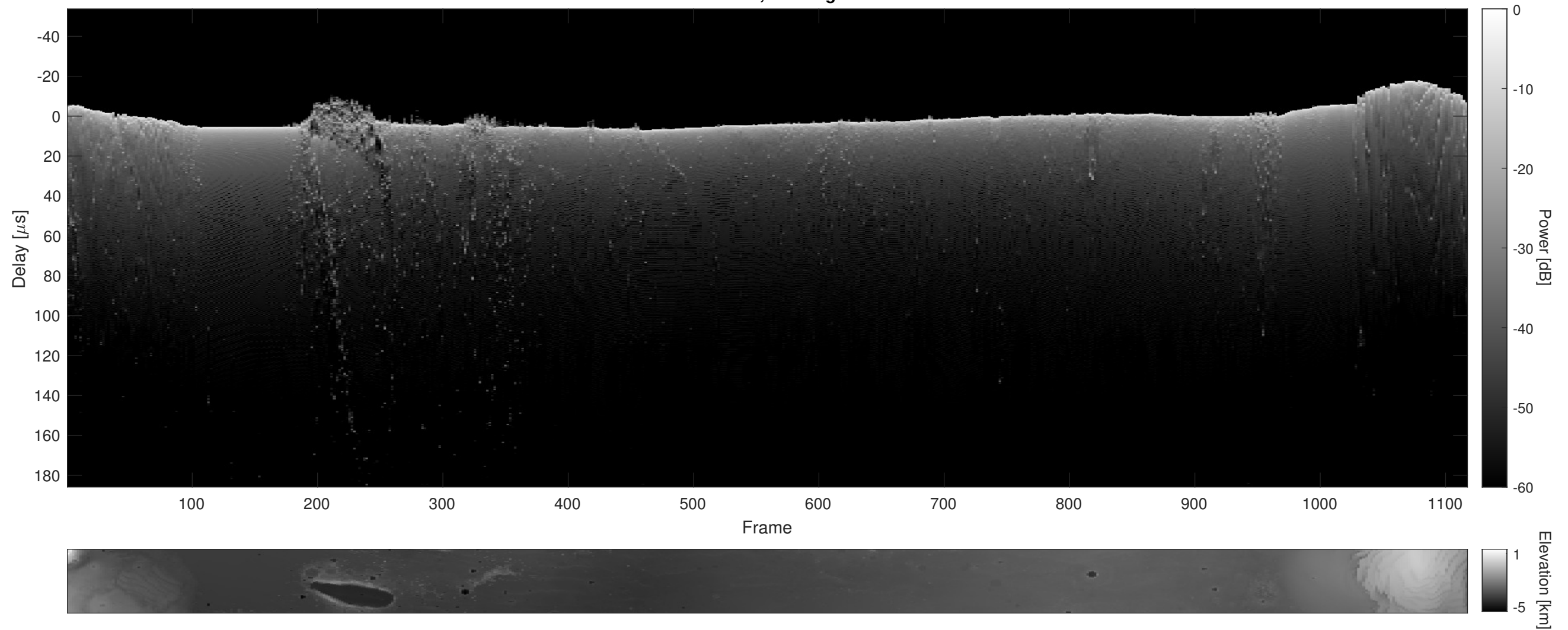
Orbit 16340, Cluttergram
