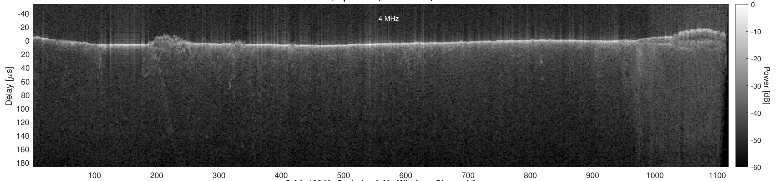
Orbit 16340, Optimized, No Window, Channel 2
