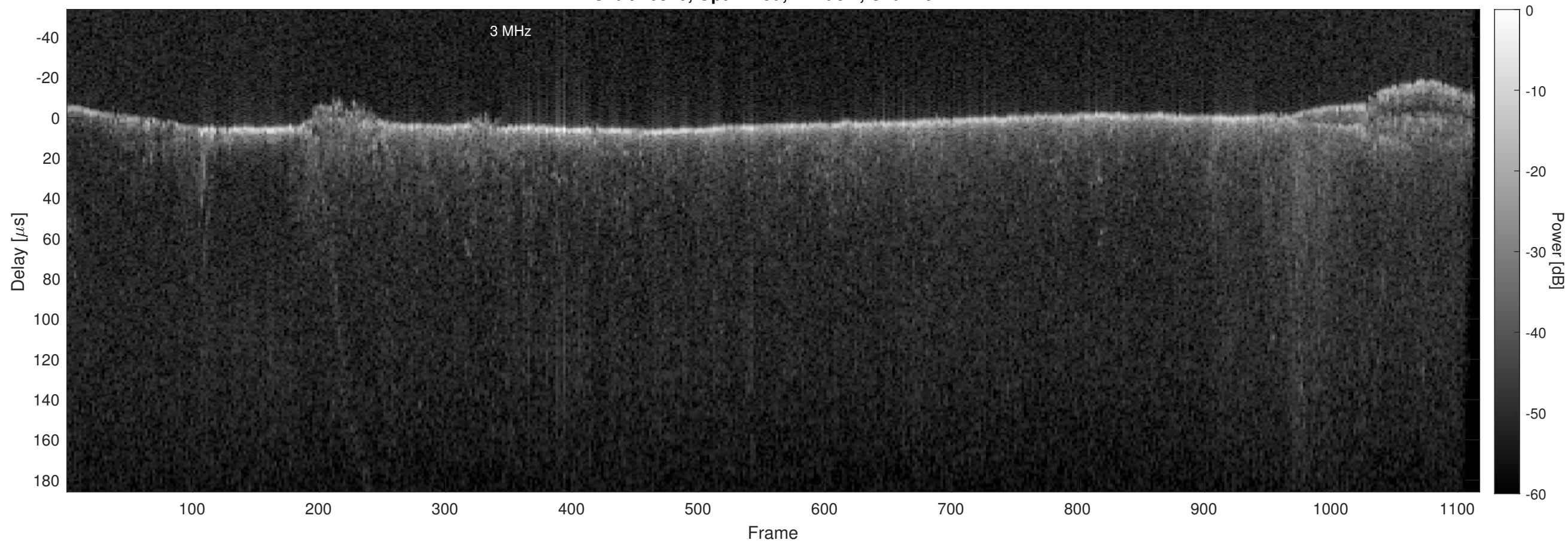
Orbit 16340, Optimized, Window, Channel 2
