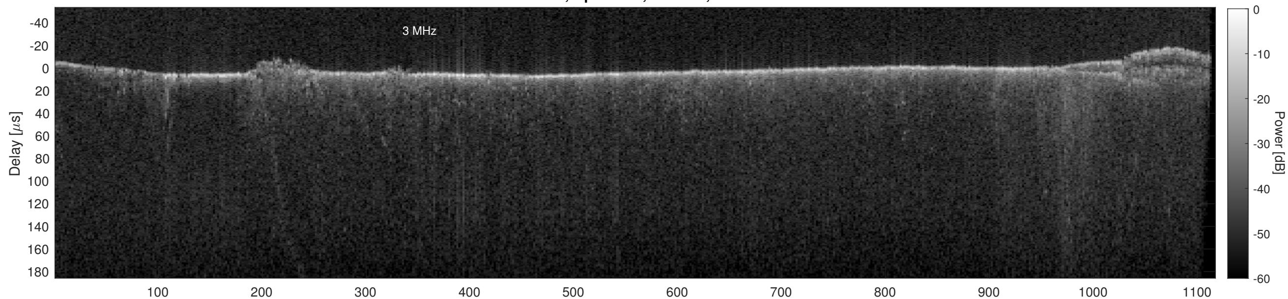
Orbit 16340, Cluttergram
